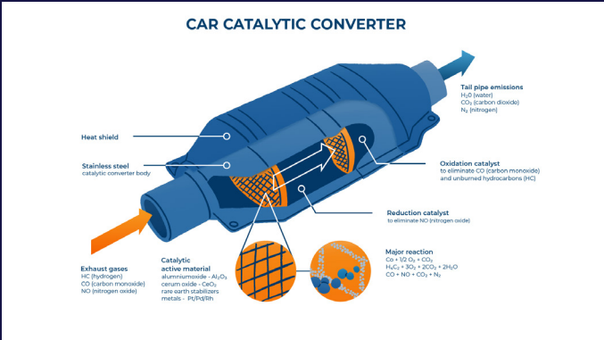
car Catalytic Converter diagram for blog, illustrated in Procreate, designed in Illustrator, 2024.
